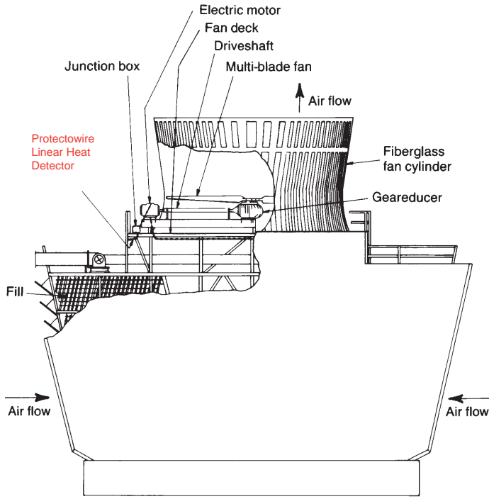
Figure 7 Partial transverse section
