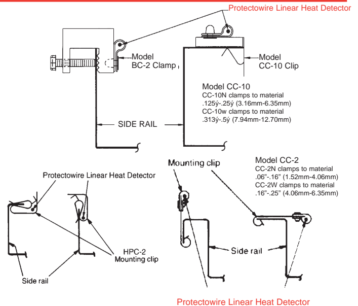
Figure 10B Typical Cable Tray Mountings
