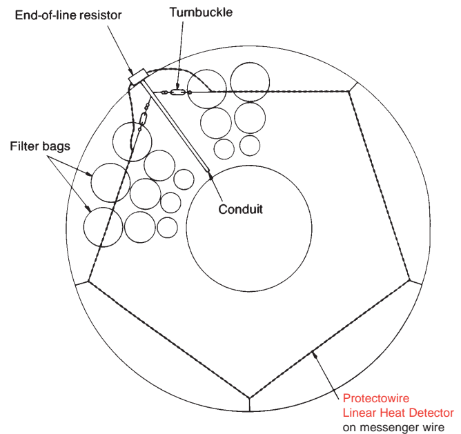
Figure 6B Top view horizontal section
