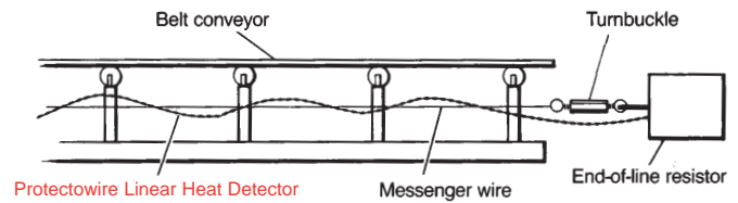
Figure 3A Side view
